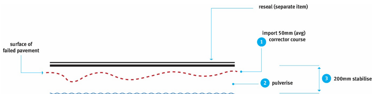
Figure 9 – In-situ stabilisation
