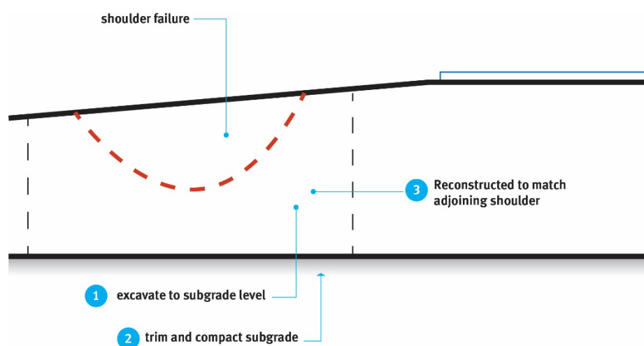
Figure 12 – Reconstruct unsealed shoulder
