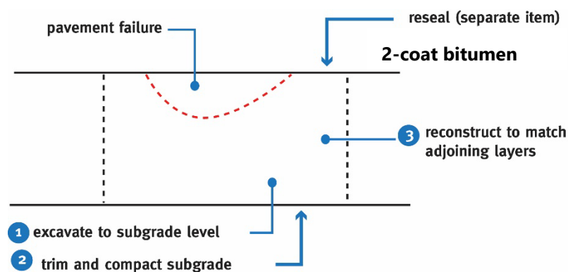
Figure 8 – Pavement repair
